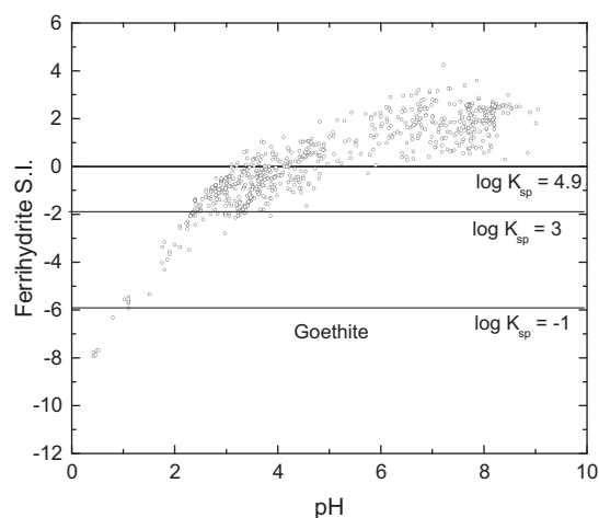
Fig. 4. Ferrihydrite [Fe(OH) 3 ] saturation indices relative to pH for 1510 screened analyses from western USA mine sites.
