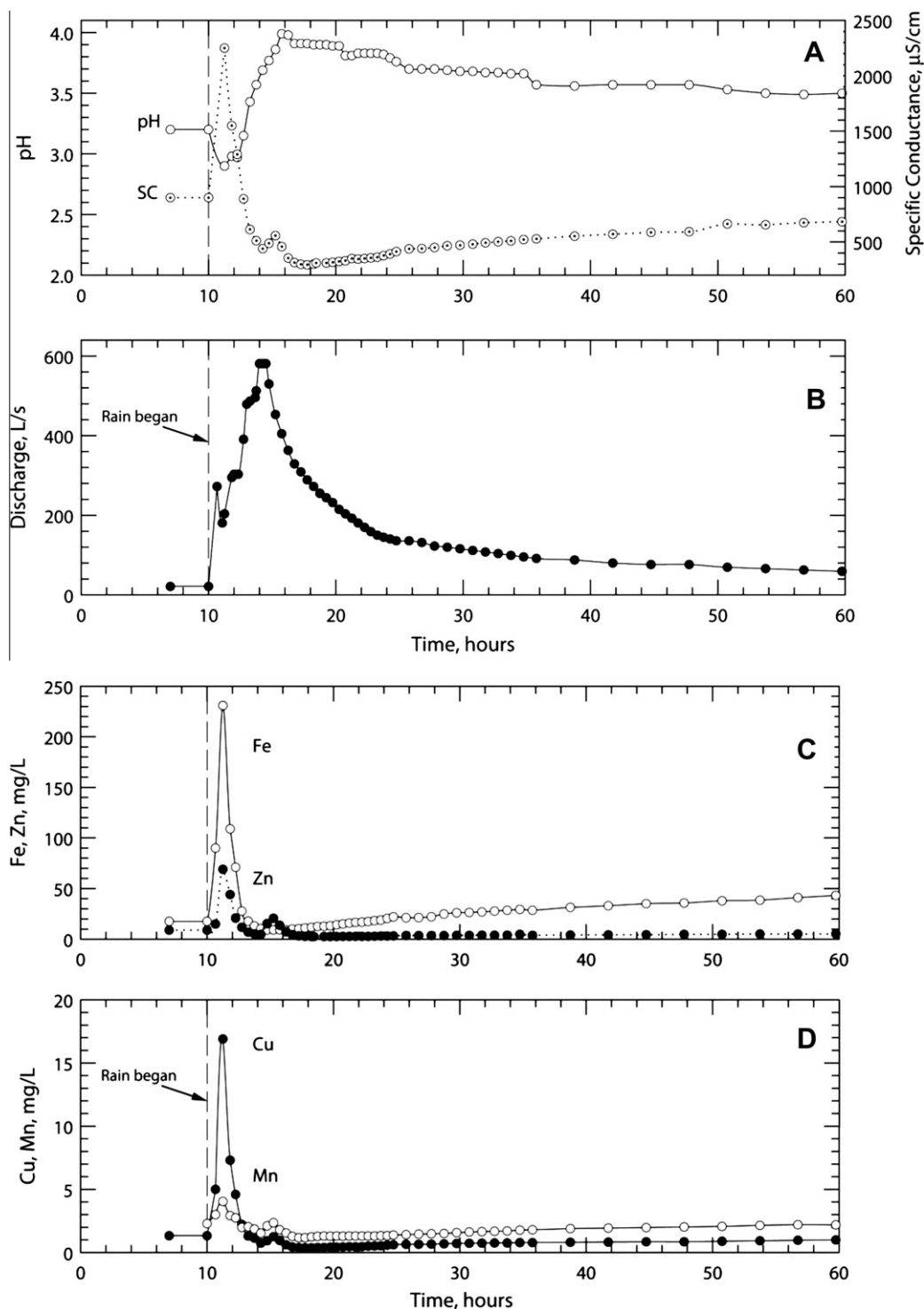
Fig. 1. Response of pH and specific conductance (A) to a rainstorm event and changing discharge of Contrary Creek, Virginia, USA (B) with consequent changes in Fe, Zn (C), and Cu, Mn (D) concentrations (modified from Dagenhart, 1980; Nordstrom, 2009).
