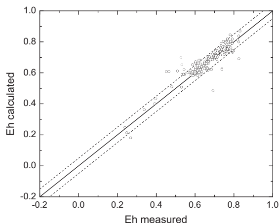
Fig. 6. Same plot as Fig. 5 with all points removed for which Fe determinations were less than 10^{-5.5} m and Fe(III) determinations were less than 3% of the total dissolved Fe concentration.
