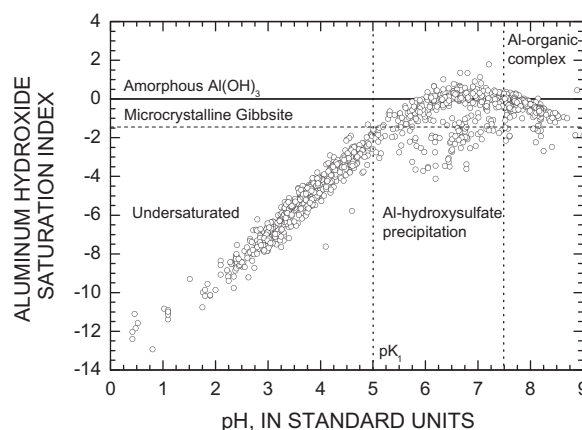
Fig. 8. \text{Al}(\text{OH})_3 saturation indices relative to pH for the same samples shown in Fig. 4.
