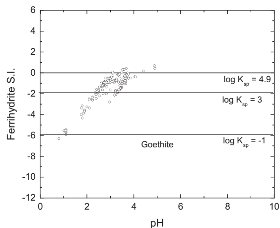
Fig. 7. Same plot as Fig. 4 after removing all points below detection limits of Fe(III) and of redox electrode measurements.
