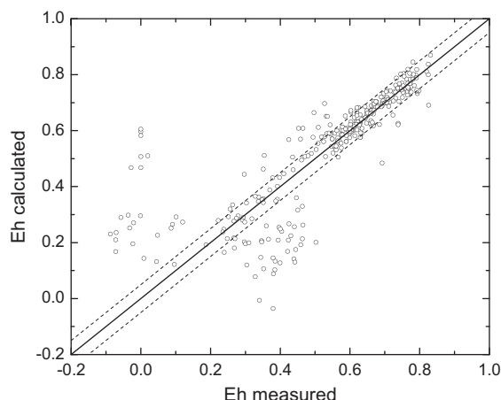
Fig. 5. Eh calculated from Fe(II/III) determinations and speciation from the WATEQ4F code substituted into the Nernst equation compared to the measured redox potential corrected for the half-cell reference potential. All values in volts. Samples are the same as those used in Fig. 4.
