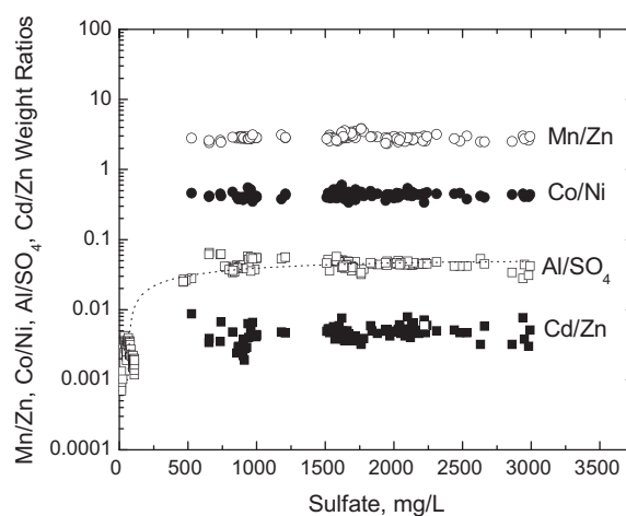
Fig. 2. Plot of Mn/Zn, Co/Ni, Al/SO 4 , and Cd/Zn weight ratios for the Straight Creek aquifer. The pH ranges from 3 (with \text{SO}_4^{2-} concentration about 2500–3000 mg/L) at the headwaters to 4 (with \text{SO}_4^{2-} concentrations about 500–1000 mg/L) at the downgradient end of the aquifer (data from Naus et al., 2005). Dotted line represents Al/SO 4 ratios for the Red River downstream from the Straight Creek catchment, northern New Mexico, USA.
