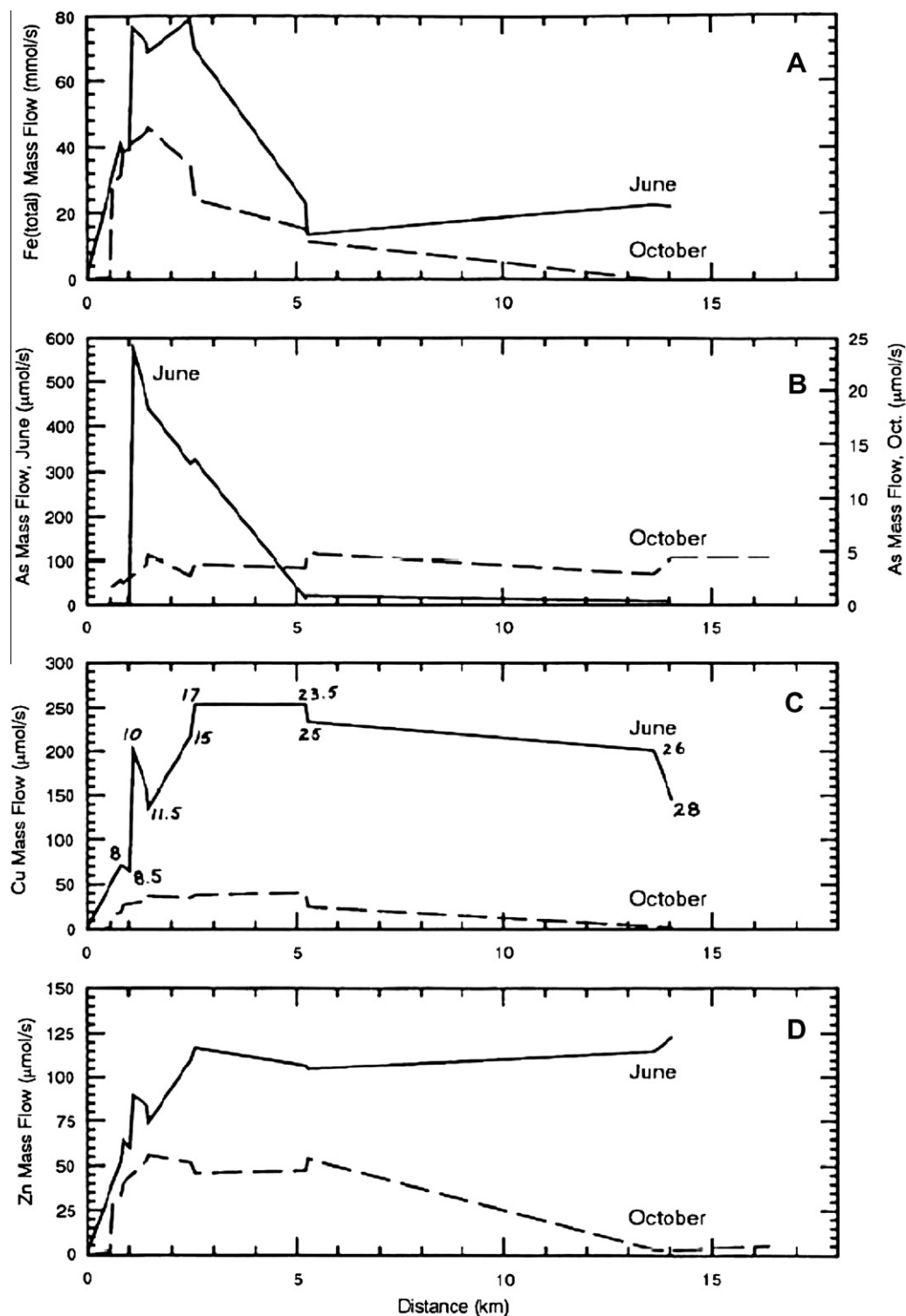
Fig. 3. Mass flow for Fe (a), As (b), Cu (c) and Zn (d) under two different flow regimes for the Leviathan Creek/Bryant Creek, southeastern California, drainage system (from Webster et al., 1994). Most of the acid mine drainage from the Leviathan mine enters the main drainage within the first kilometer downstream from the mine.
