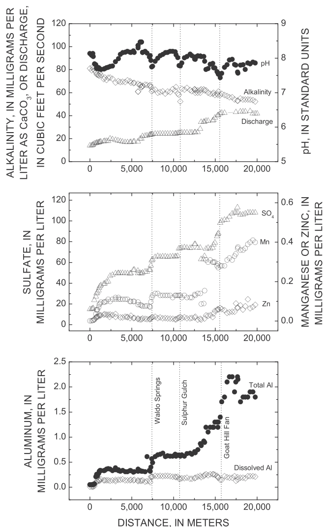
Fig. 9. Profile of pH, alkalinity, discharge, and Mn, Zn, \text{SO}_4 , total Al, and dissolved Al concentrations along the central portion of the Red River, northern New Mexico, USA (from Nordstrom, 2005, 2008). (N.B. – 1 Cubic foot = 0.0283 \text{ m}^3 ).
